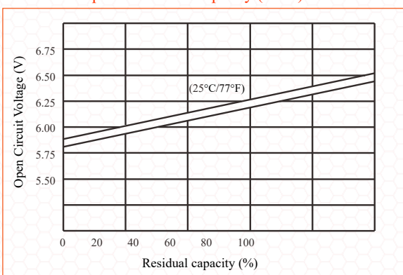
Relationship for OCV and capacity (25°C)
